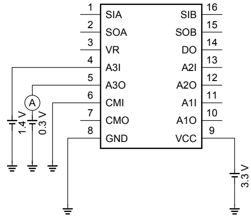
(18) Window comparator
