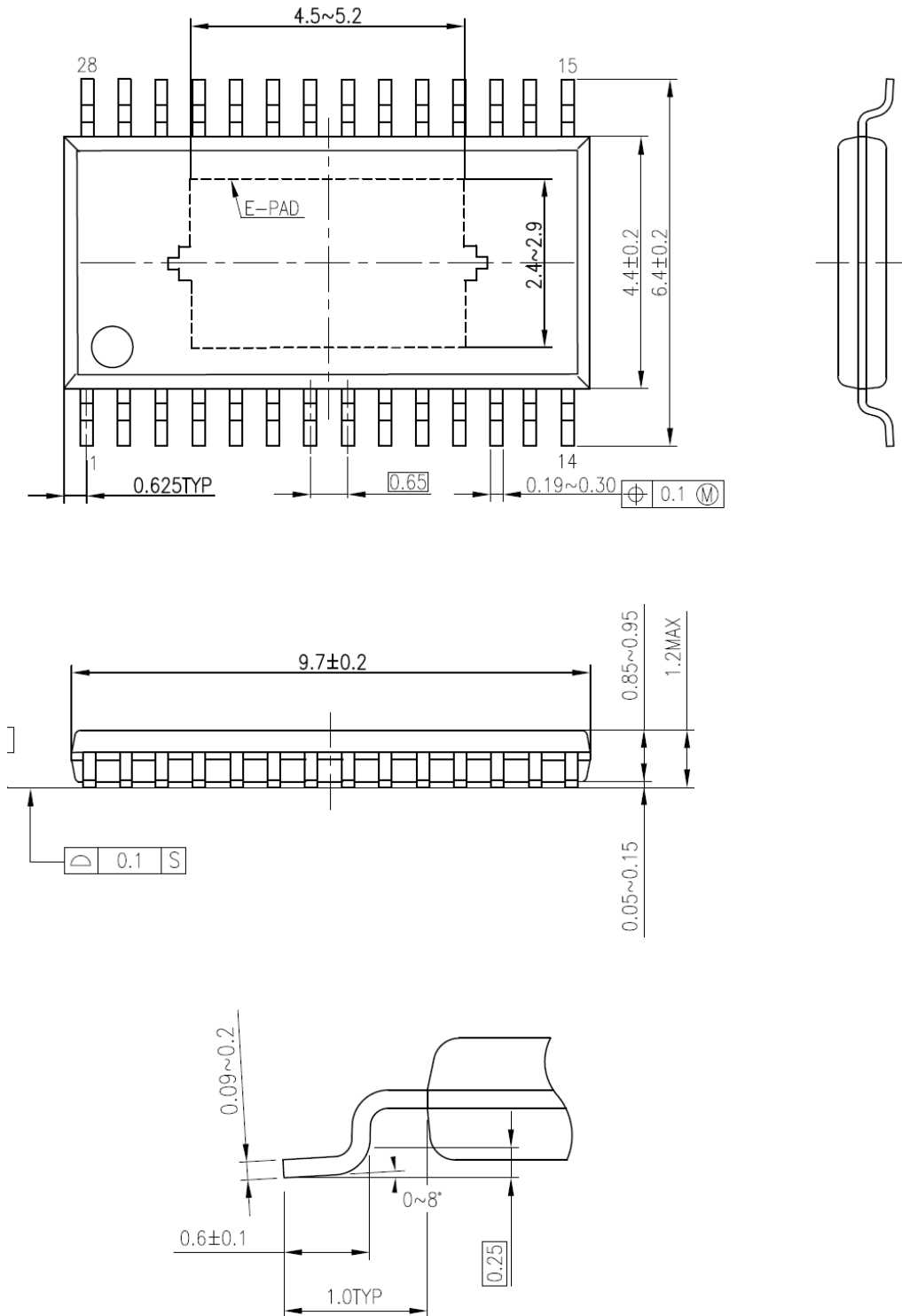
Figure22 Package Dimensions
