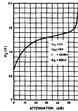
Fig. 4 Control voltage v. attenuation
