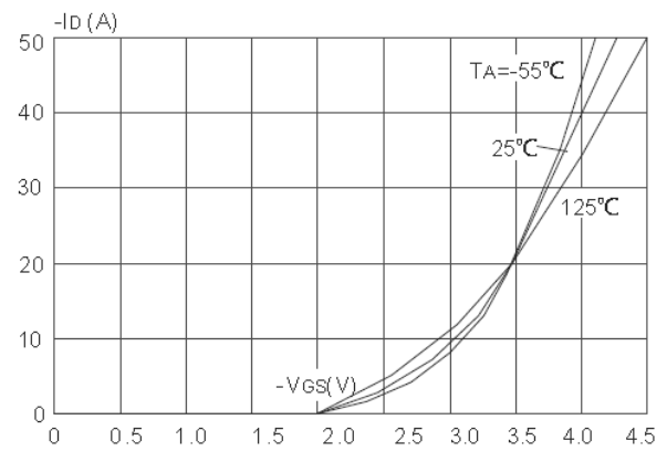
Fig 6 Transfer Characteristics
