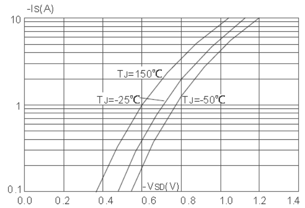
Fig 4 Body-Diode Characteristics
