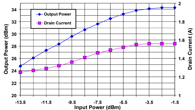
Power Transfer Curve and Drain Current at 14.25 GHz Biased at V_d = 8V and V_g = -0.2V (typical)
