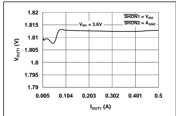
FIGURE 2-11: V_{OUT1} vs. I_{OUT1} ( V_{OUT1} = 1.8V ).
