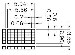
DETAIL DOTS SCALE 2:1
