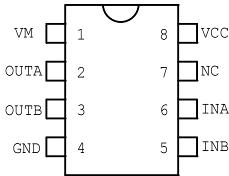
(SOP-8) TH2466A
