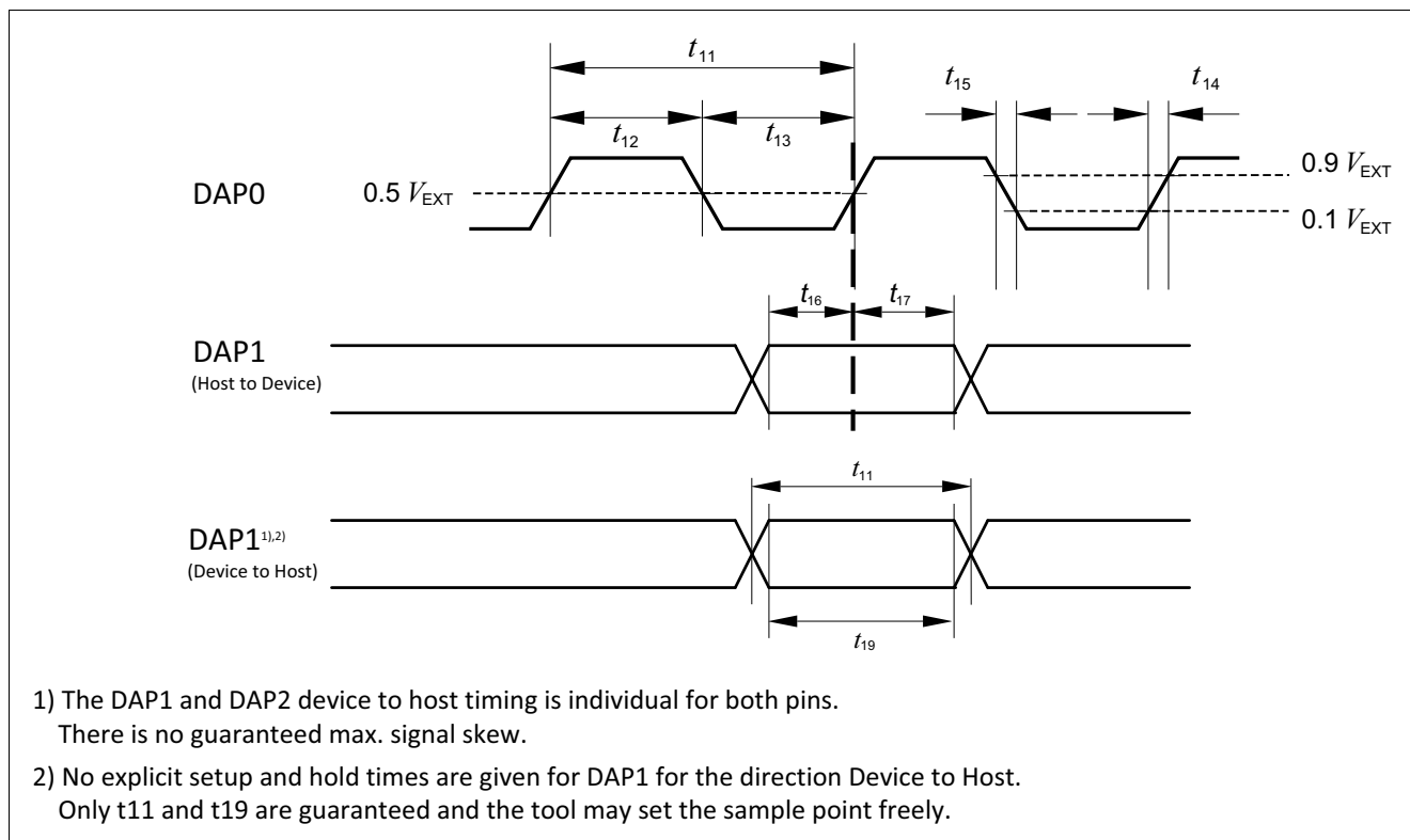
Figure 3-12 DAP Timing
