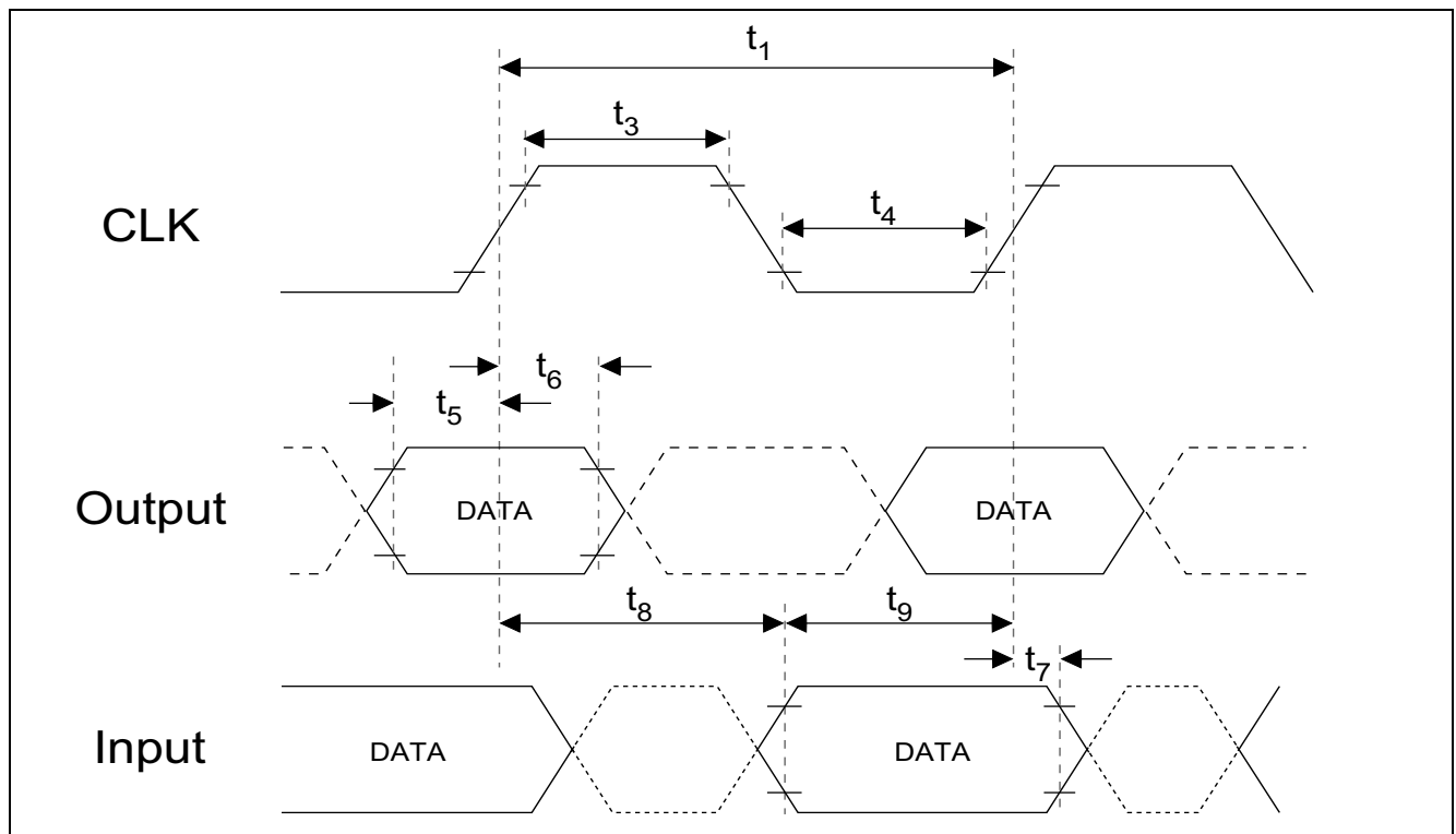
Figure 3-24 SDMMC Timing
