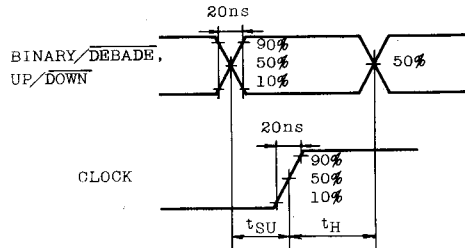
WAVEFORM 7
