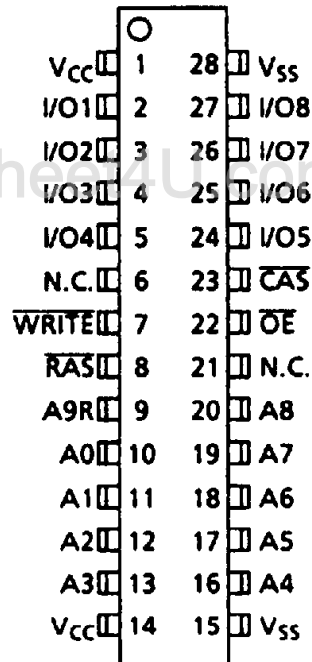
Plastic TSOP (Normal Bend Type)
