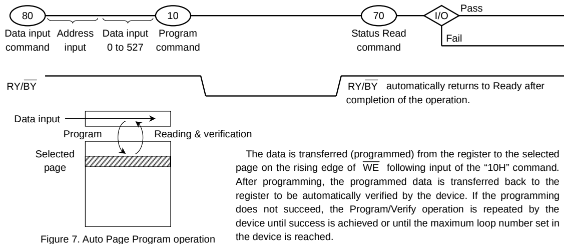
Figure 7. Auto Page Program operation
