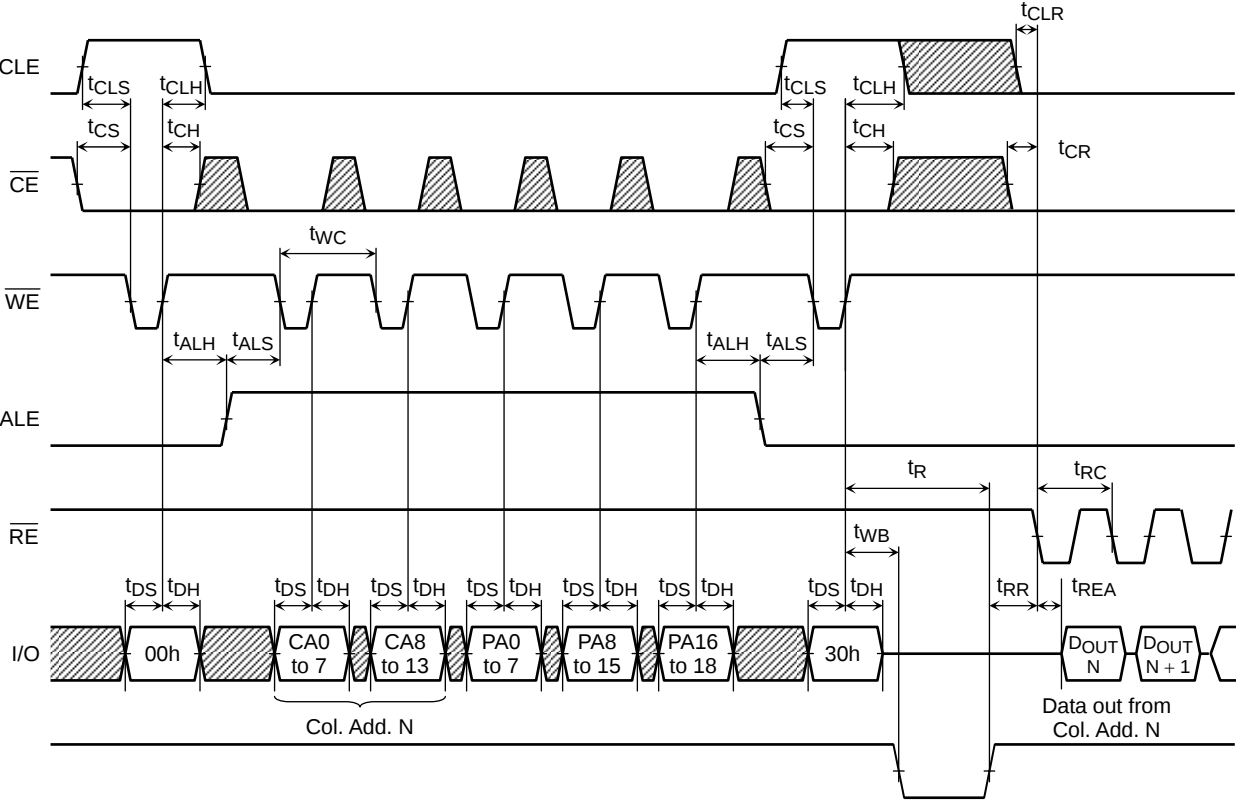
Read Cycle Timing Diagram
