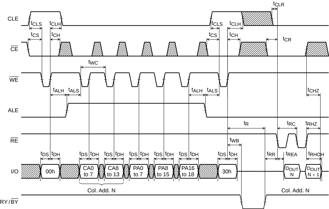
Read Cycle Timing Diagram: When Interrupted by \overline{CE}
