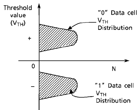
Figure 19. V_{TH} Distribution for "0" and "1" data cells
