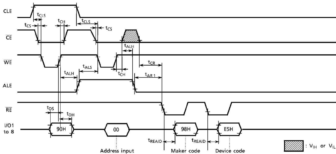
ID Read Operation Timing Diagram
