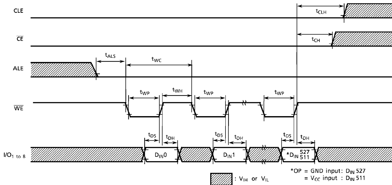
Data Input Cycle Timing Diagram
