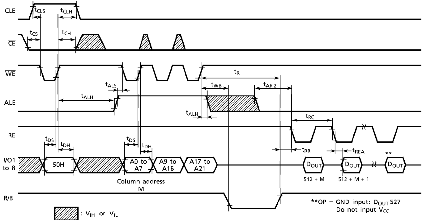
Read Cycle (3) Timing Diagram
