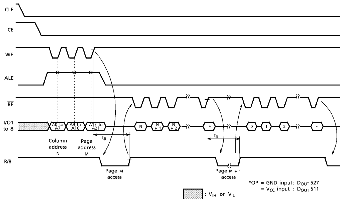
Sequential Read Timing Diagram
