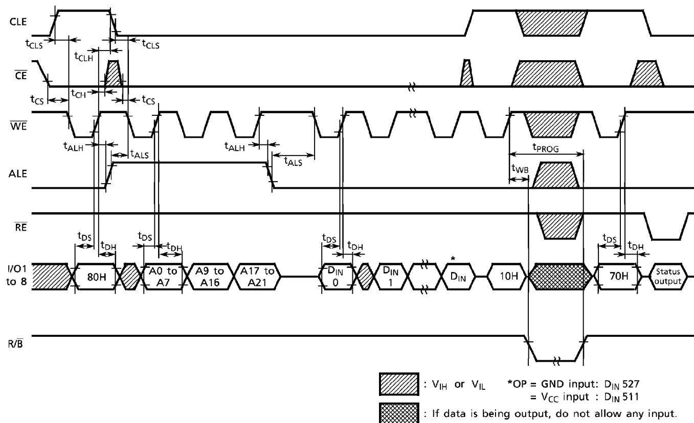
Auto Program Operation Timing Diagram
