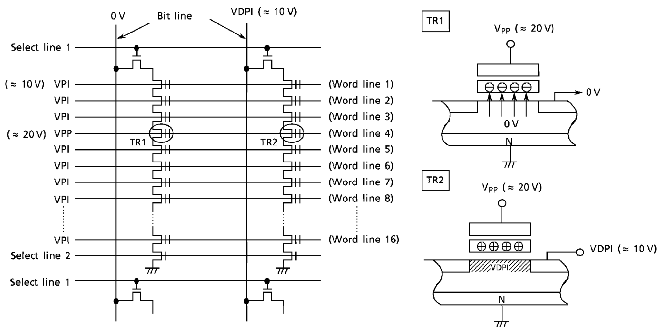
Figure 17. TC58V32FT Program Device Physics
