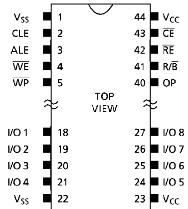
Figure 1.: TC58V32FT Pinout
