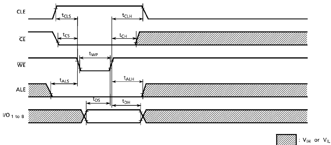
Command Input Cycle Timing Diagram
