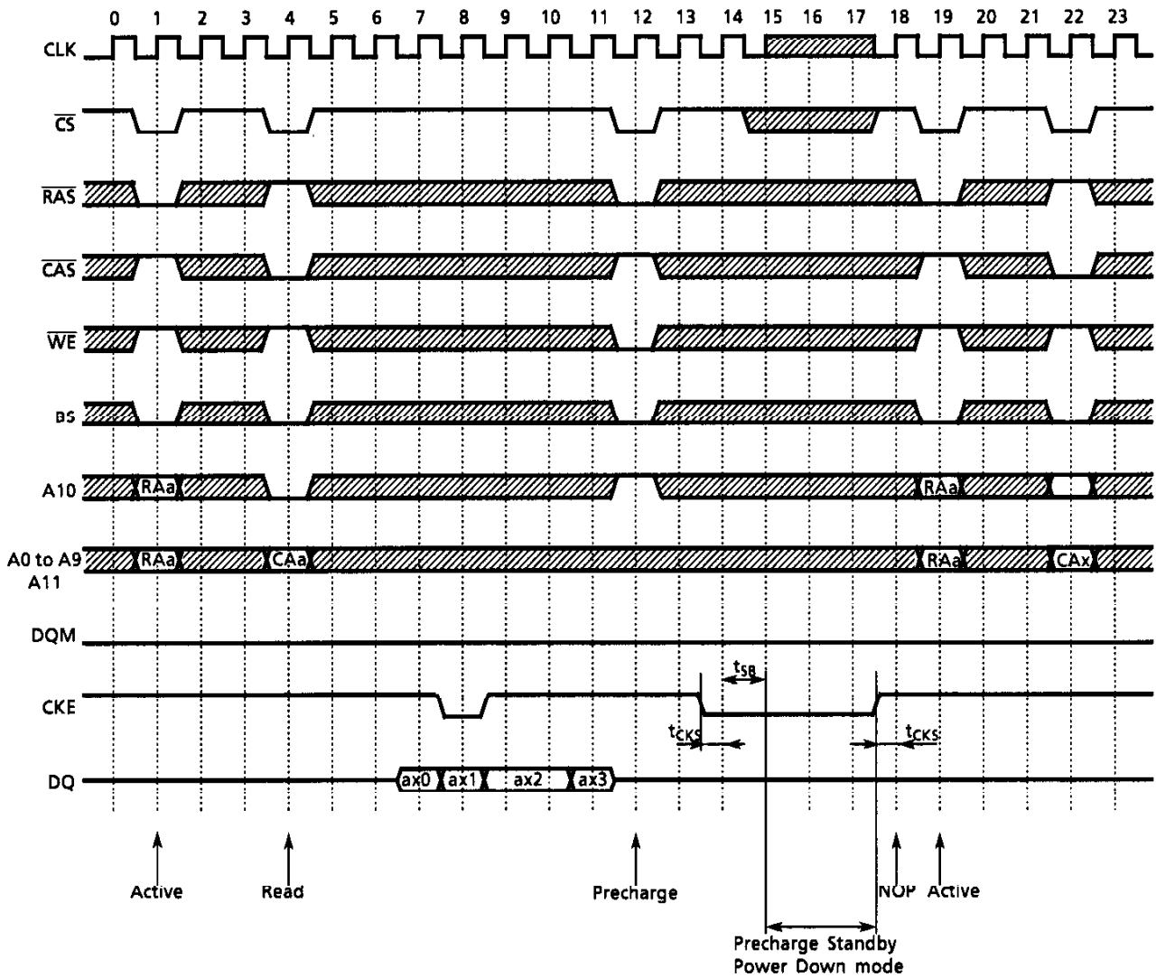
Figure 13. Power Down Mode
