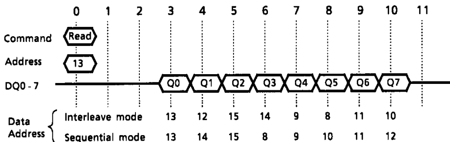
Read Cycle \overline{\text{CAS}} Latency = 3
