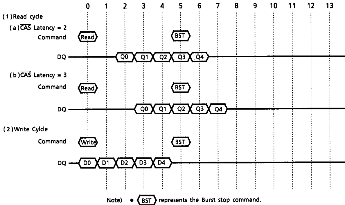
Figure 10. Timing chart for Burst Stop cycle (Burst stop command)
