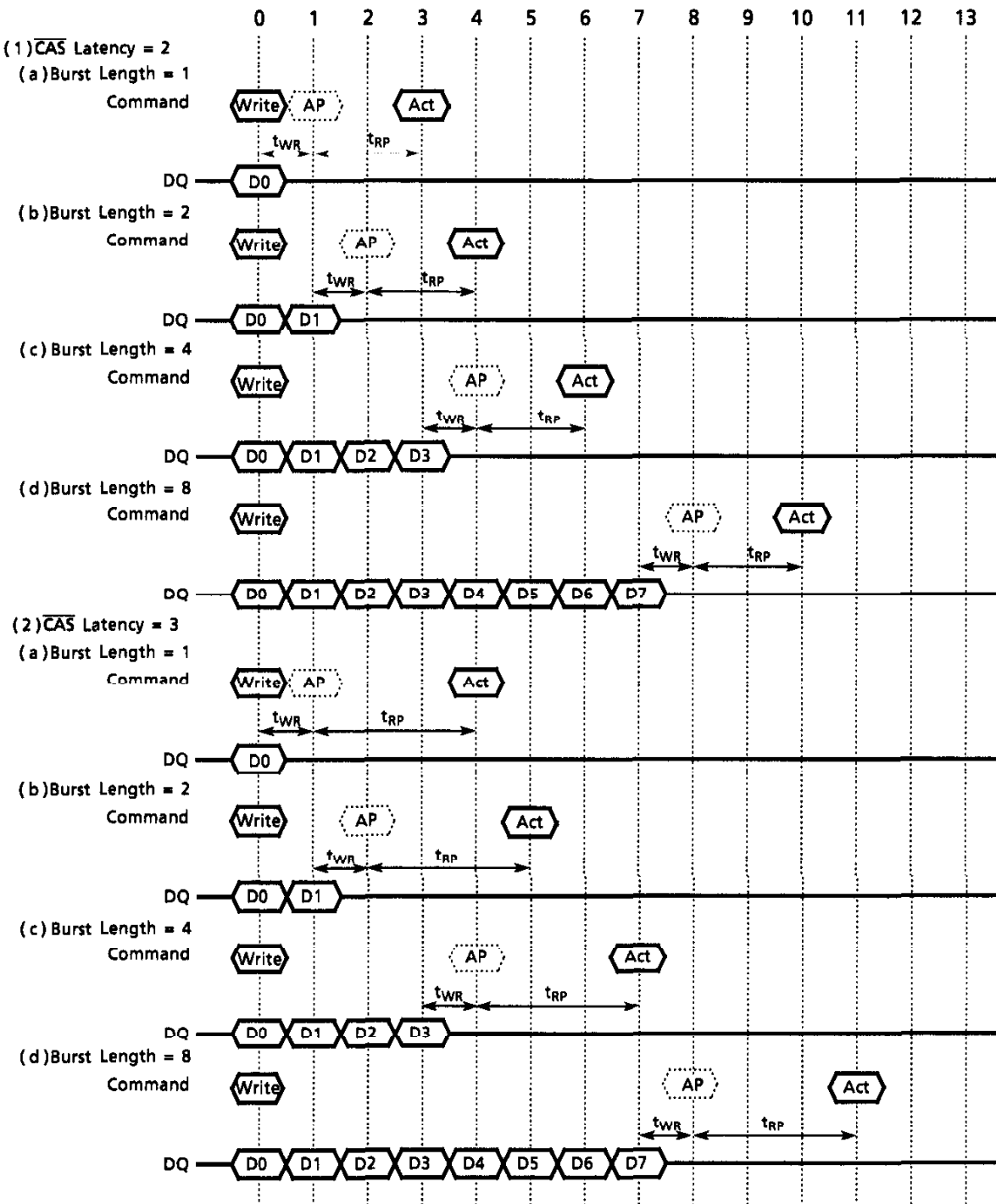
Figure16. Auto Precharge timing (Write cycle)
