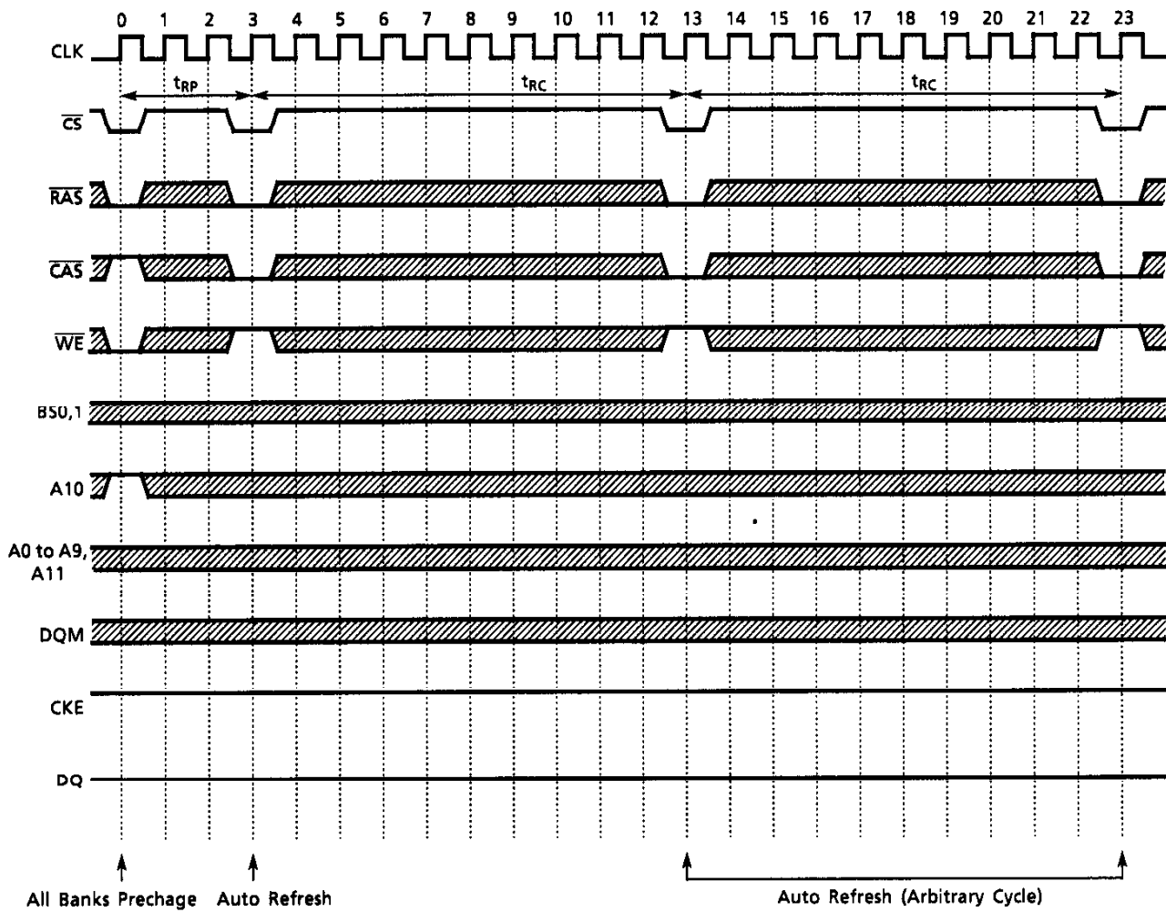
Figure 11. Auto Refresh cycle
