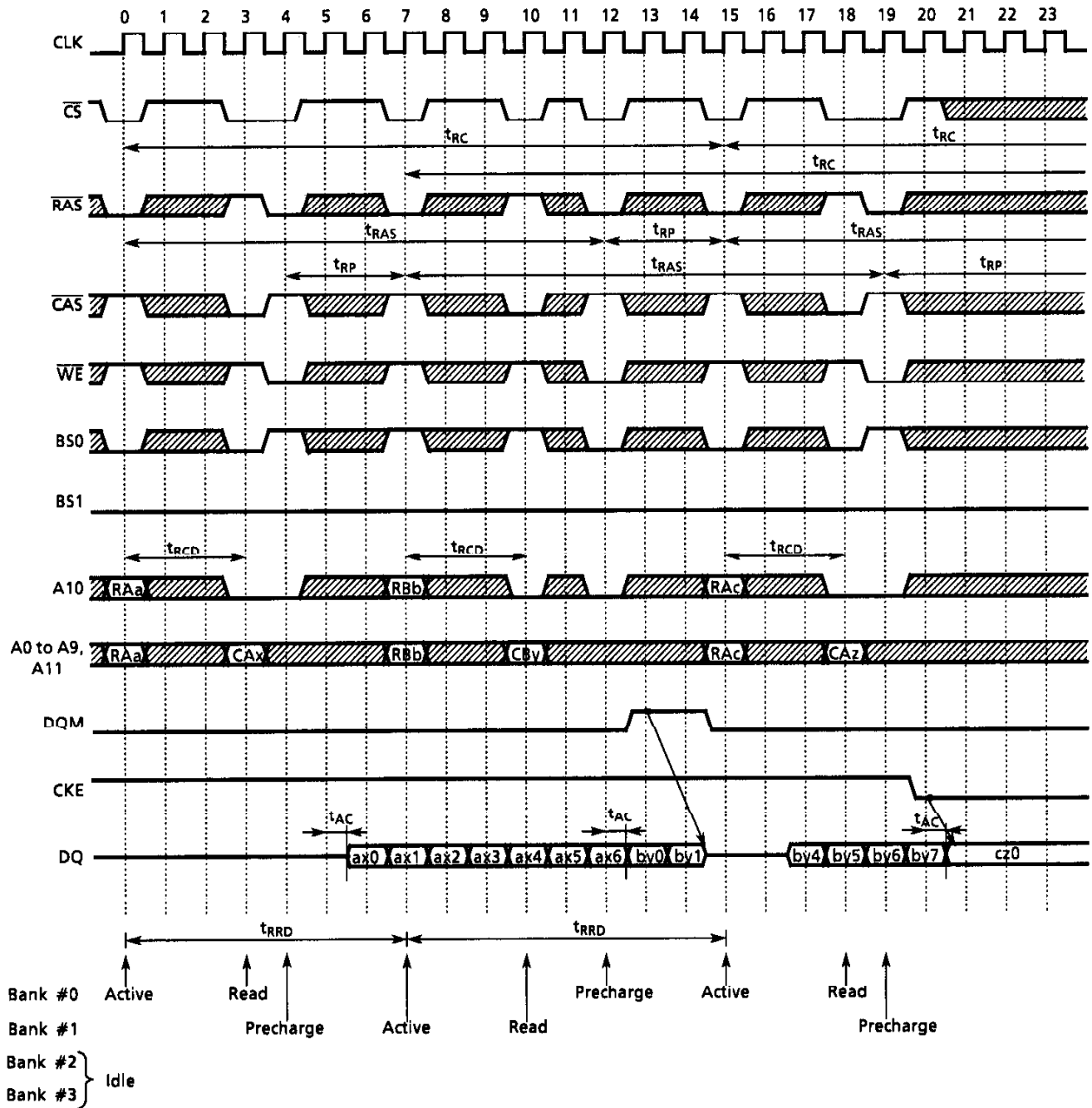
Figure 3. Interleaved Bank Read (Burst Length=8, CAS Latency=3)
