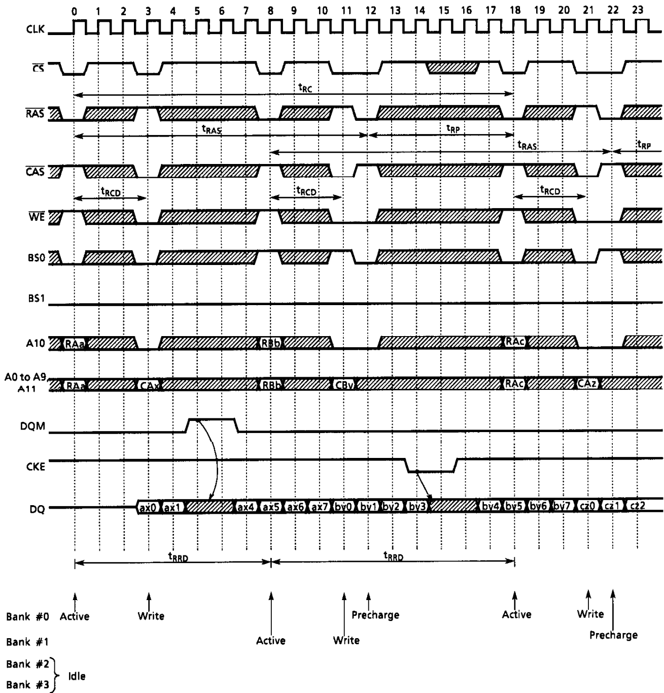
Figure 5. Interleaved Bank Write (Burst Length=8)
