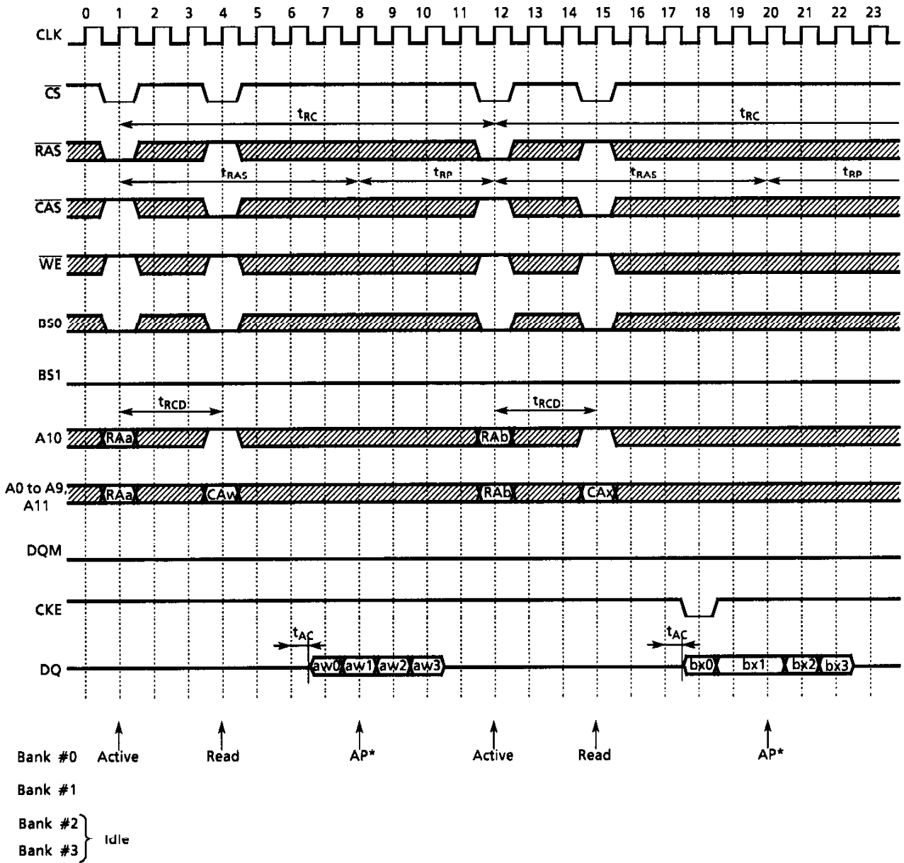
Figure 9. Auto Precharge Read (Burst Length=4, \overline{CAS} Latency=3)
