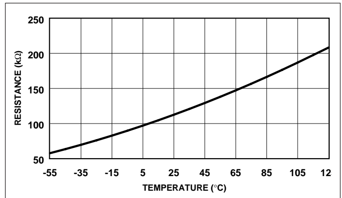
Figure 2. TC620 Sense Resistors vs. Trip Temperature
