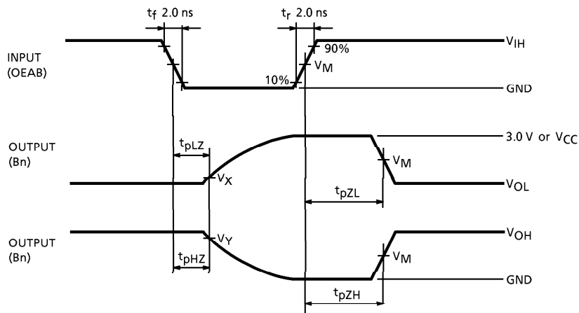
Fig.6 t_{pLZ} , t_{pHZ} , t_{pZL} , t_{pZH}
