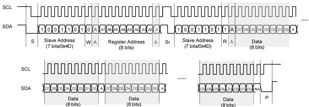
Figure 8-13 Continuous read mode
