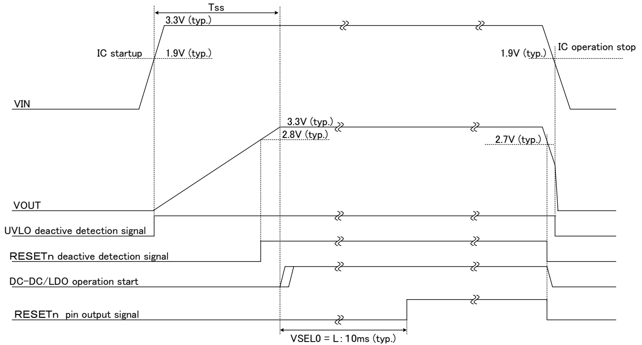
Figure 8-4 RESETn deactive/detection operation (VSEL0 = "L", MODE_SEL = "L")
