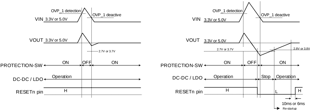
Figure 8-2 OVP_1 operation
