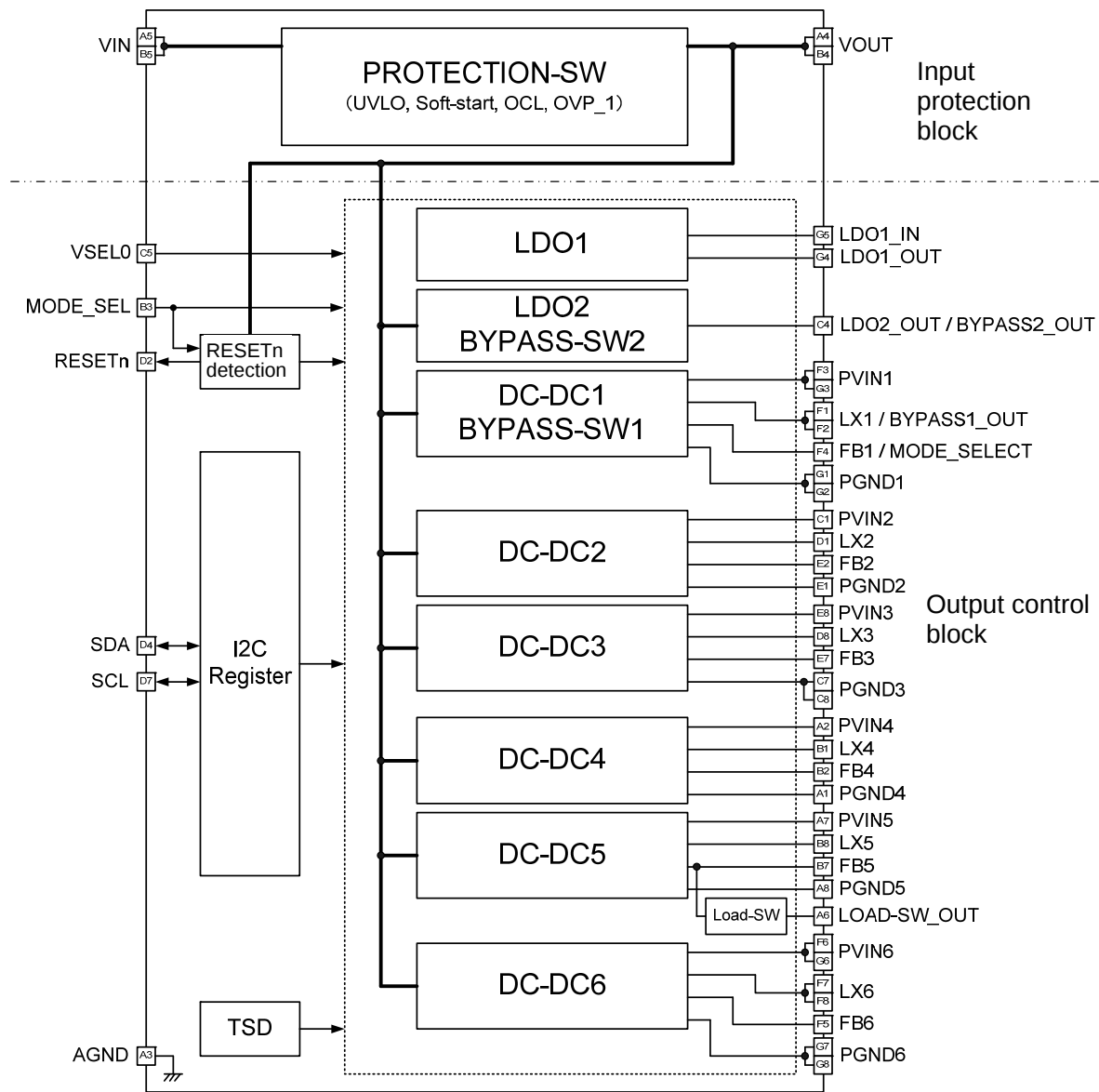
Figure 7-1 Block diagram
