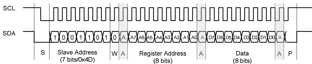
Figure 8-10 Single write mode
