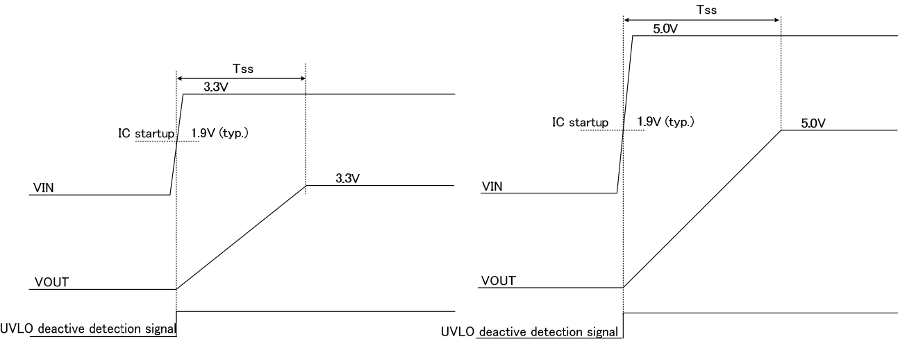
Figure 8-3 Soft start
