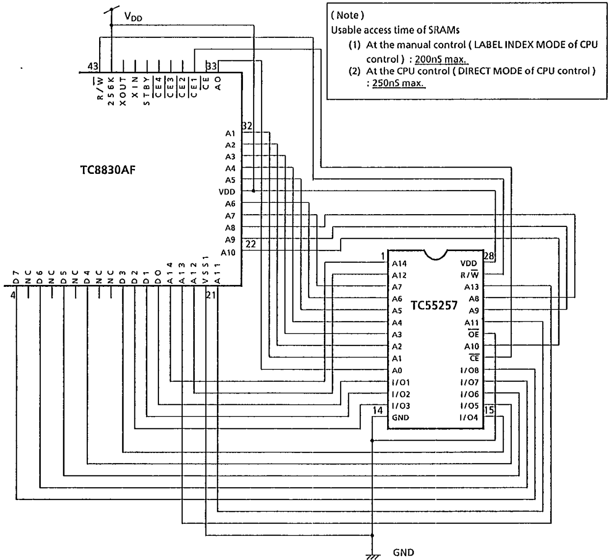
Fig.5.40 Connection of SRAM ( In case of 256K DRAM )
