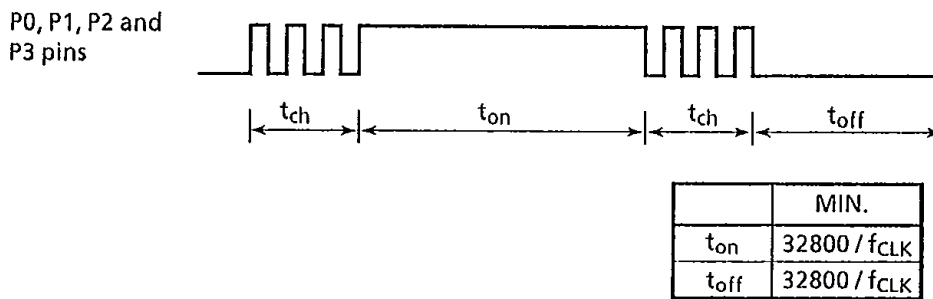
Fig.5.10 Chattering elimination circuit
