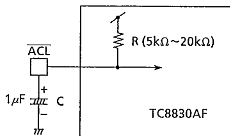
Fig.5.30 Power on reset circuit
