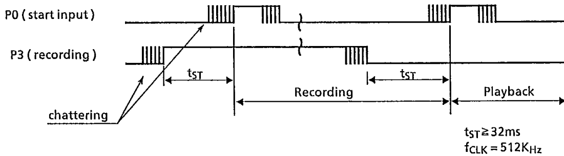
Fig.5.6 Timing of change at recording / playback
