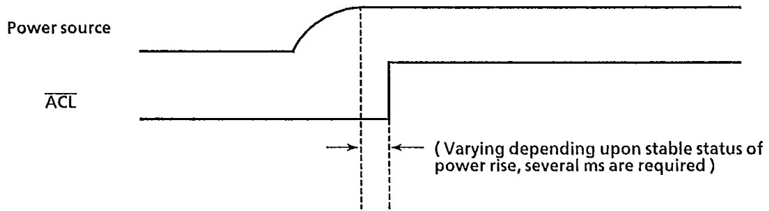
Fig. 5.32 System initialization by CPU control
