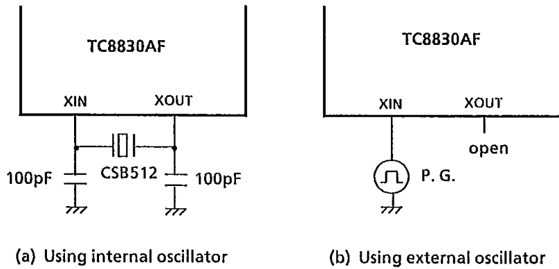
Fig.5.41 Oscillator
