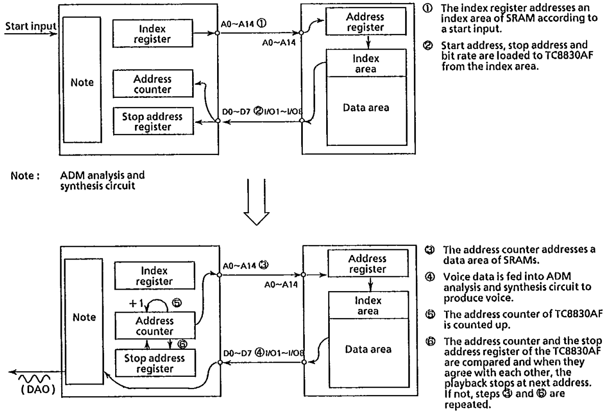
Fig.5.27 Playback
