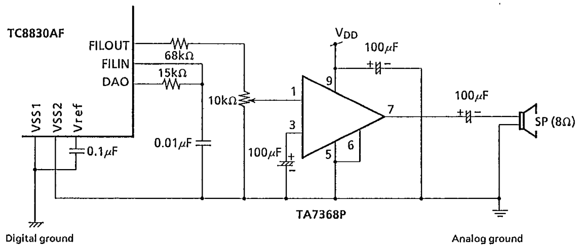
Fig.5.45 Connection of audio amplifier
