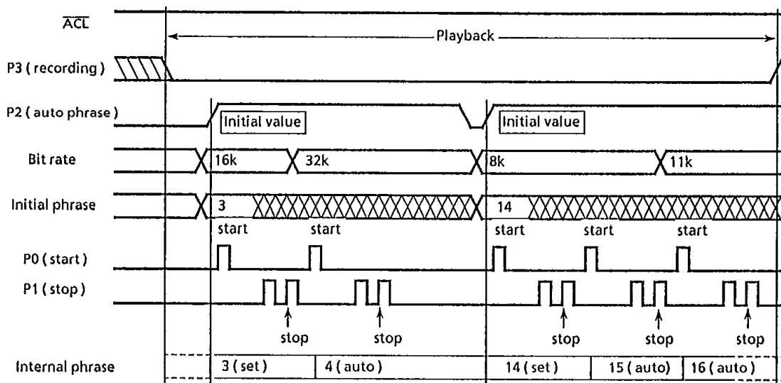
Fig.5.8 Auto phrase playback
