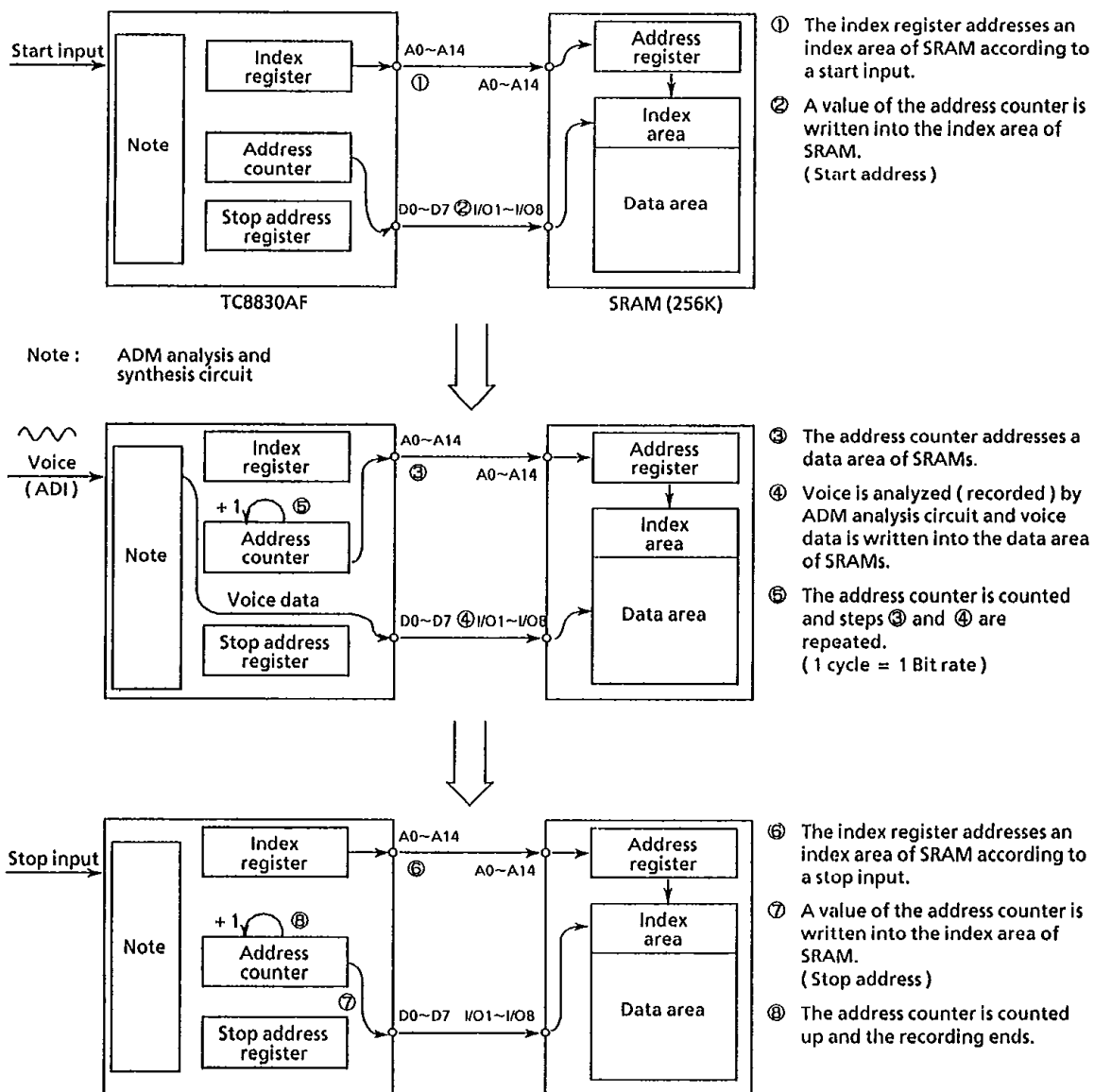
Fig.5.26 Recording
