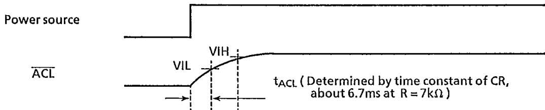
Fig. 5.31 A̅CL input at power on reset
