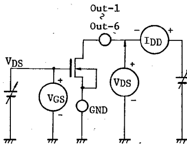
TEST CIRCUIT
