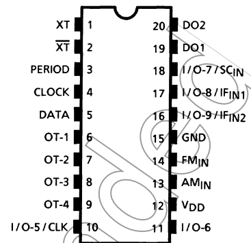
DIP-20PIN / SOP-20PIN
