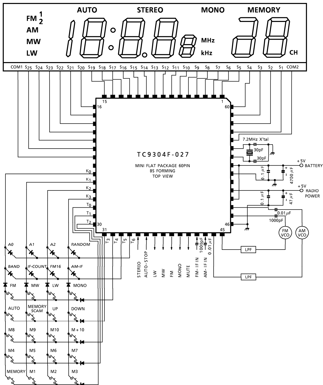
TC9304F-027 Layout
