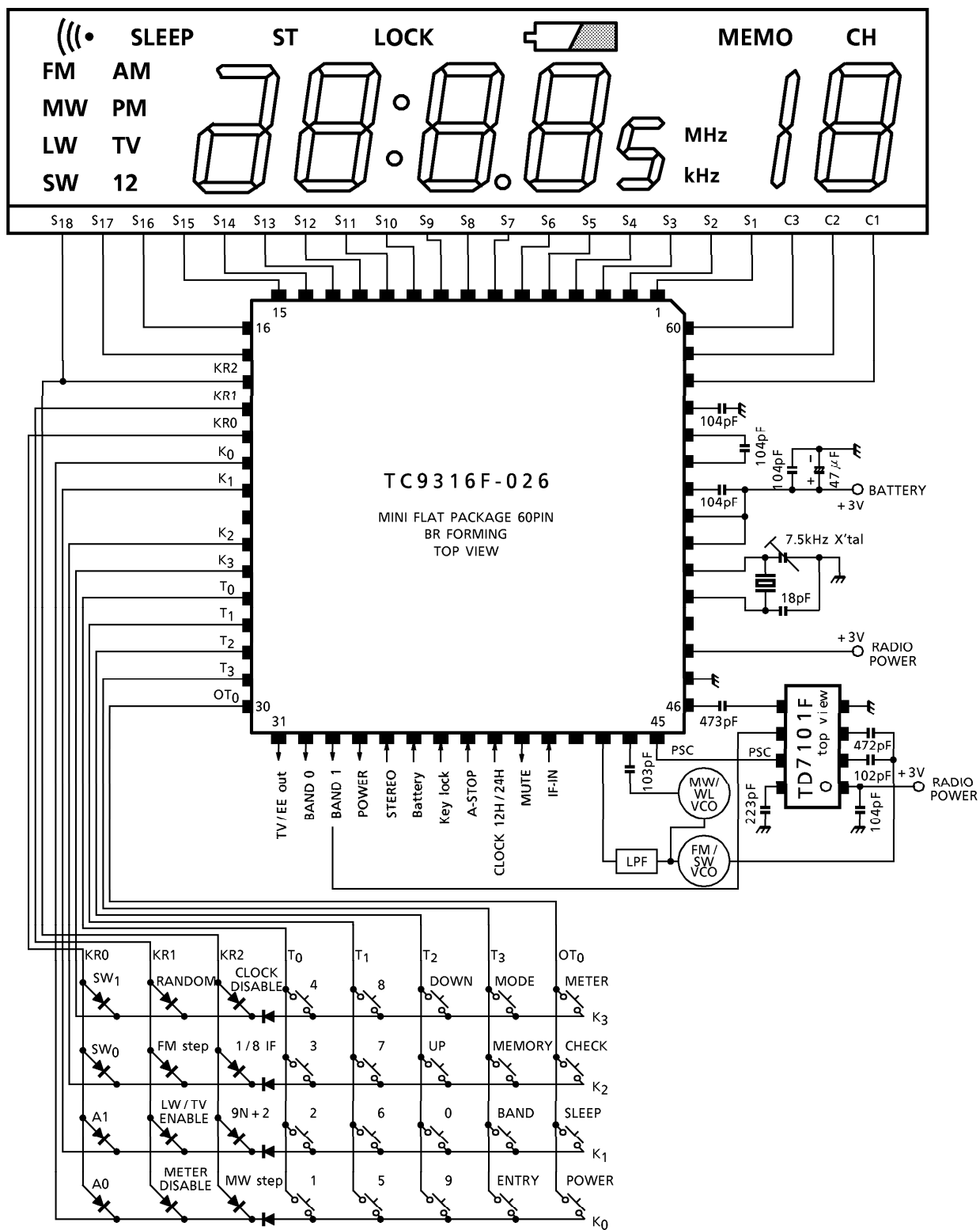
TC9316F-026 Layout
