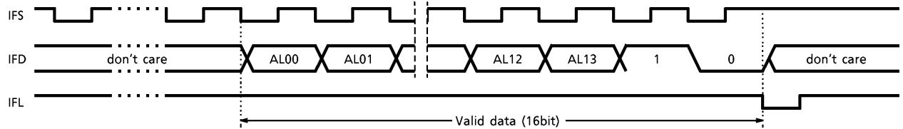
(b) Coefficient offset RAM writing (26bit command)
