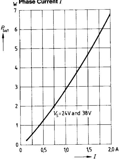
Saturation Loss P_{sat} versus Phase Current I
