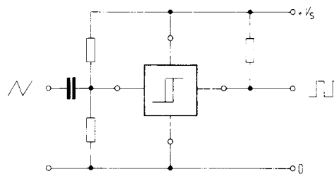
Triangle-square Converter
