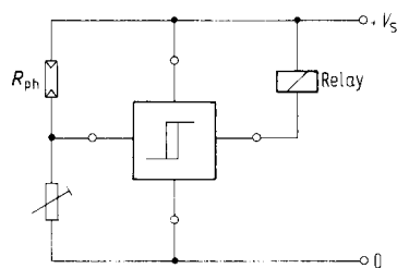
Twilight Switch (switches on light at nightfall)
