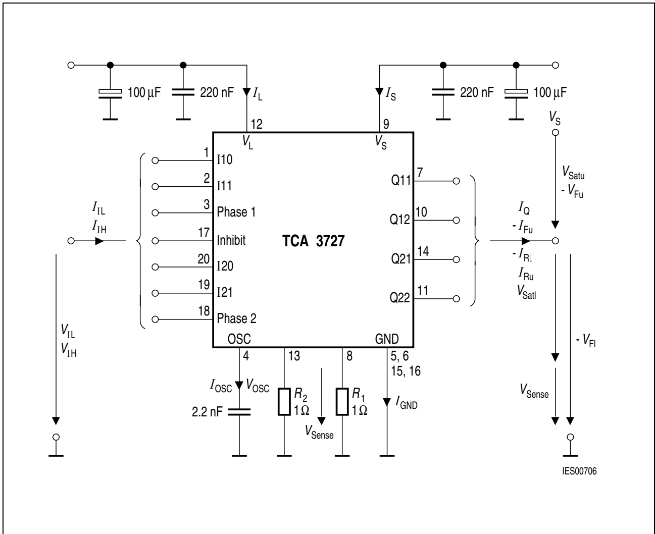
Figure 5 Test Circuit
