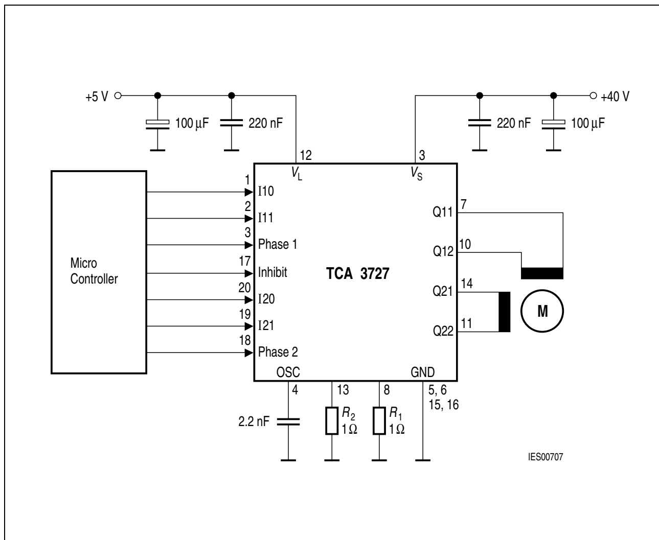
Figure 6 Application Circuit
