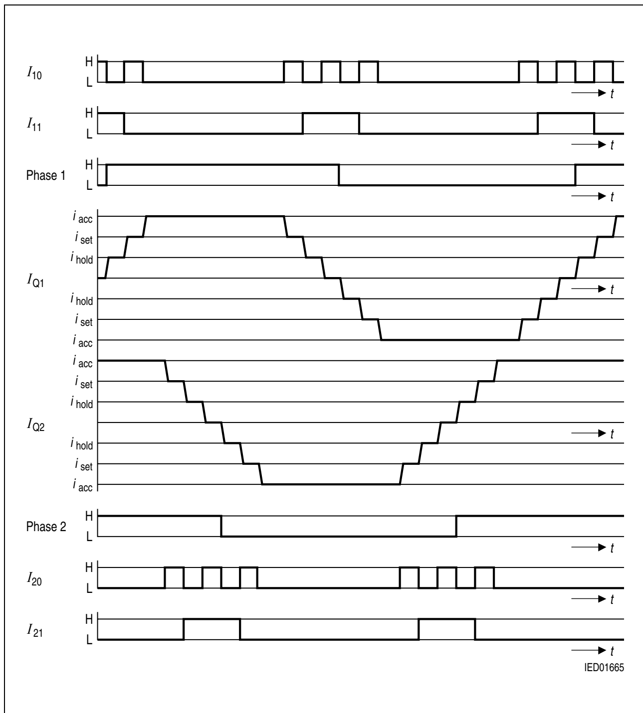
Figure 10 Mini-Step Operation
