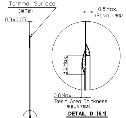
DETAIL D (5:1)
