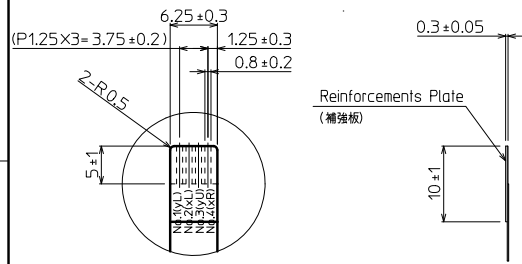
DETAIL C (2:1)
