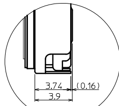
DETAIL B (5:1)
