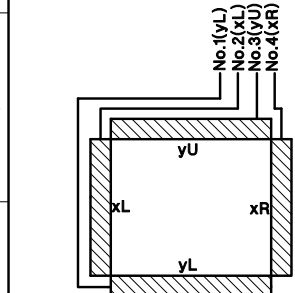
Touch Panel Pin-assign
