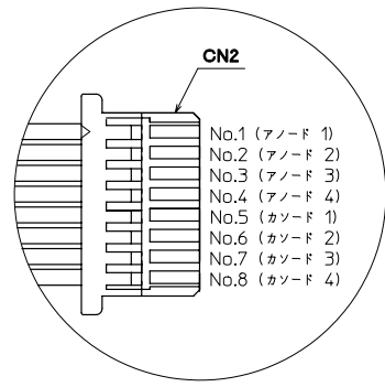
DETAIL B (5:1)
