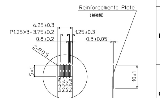
DETAIL B (2:1)
