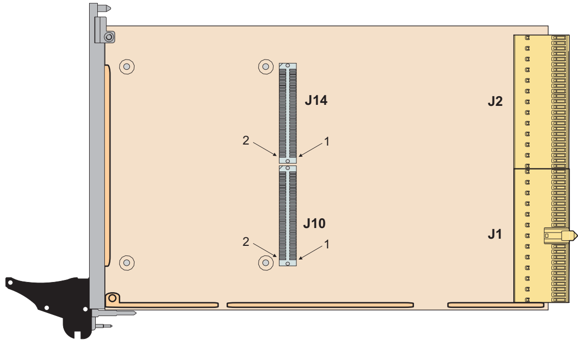
Figure 8-1 : Connector Positions
