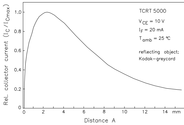
a) TCRT5000
