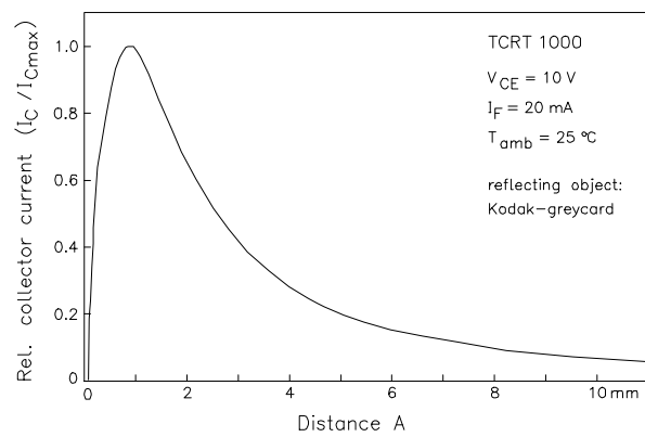
d) TCRT1000
