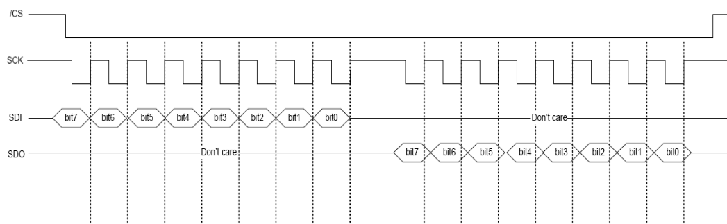
FIGURE 2-1 SPI TIMING
