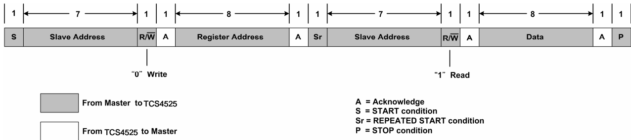
Figure12. "Read" Data Transfer Format in F/S-Mode
