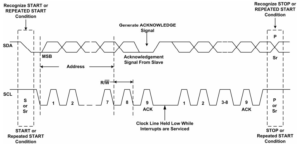
Figure10. Bus Protocol
