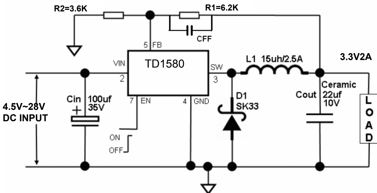
Fig11. TD1580 Typical Application Circuit (with ceramic output capacitor) @ 3.3V/2A
