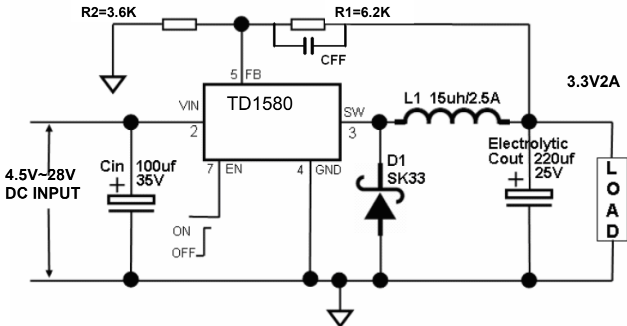
Fig9. TD1580 Typical Application Circuit @ 3.3V/2A
