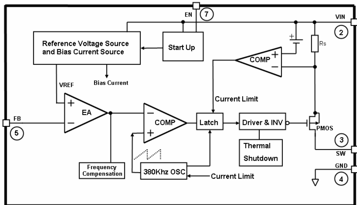
Figure 3 Function Block Diagram of TD1580
