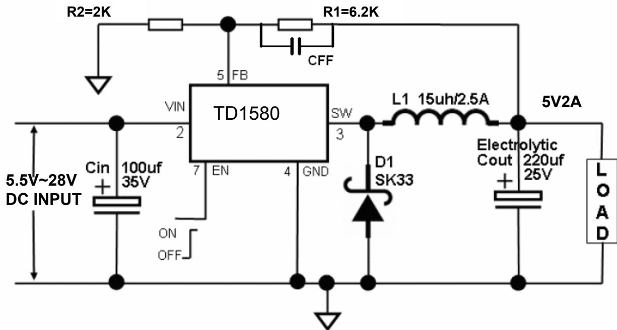
Fig8. TD1580 Typical Application Circuit @ 5V/2A
