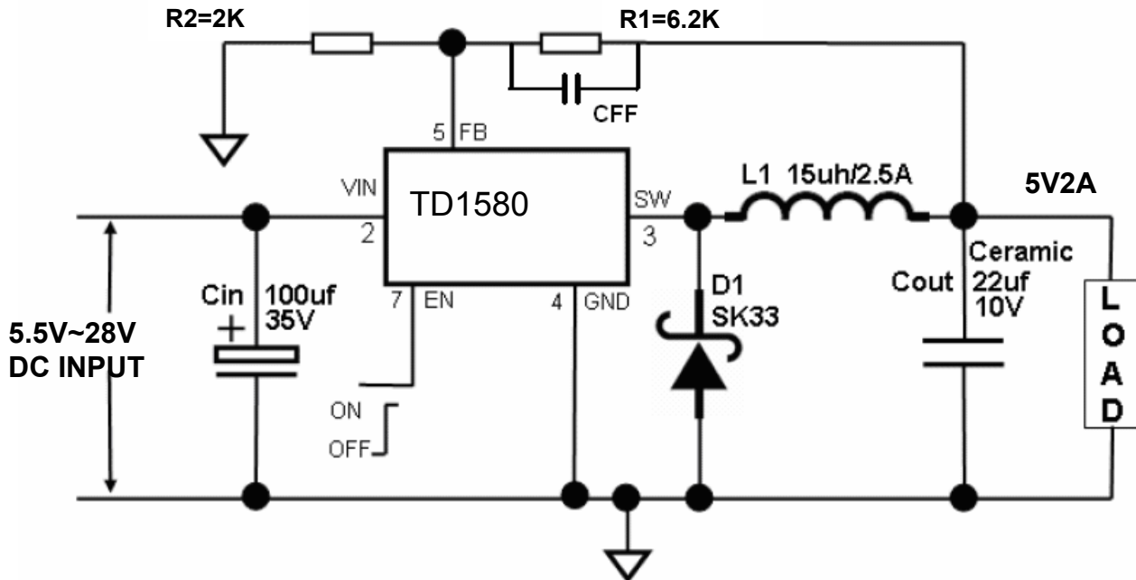
Fig10. TD1580 Typical Application Circuit (with ceramic output capacitor) @ 5V/2A
