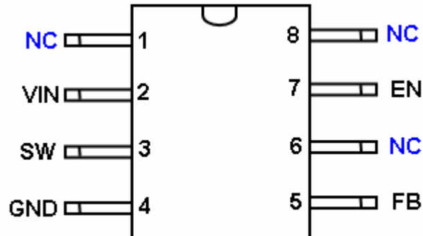
Figure 2 Pin Configuration of TD1580 (Top View)
