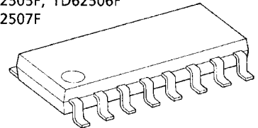
SOP16-P-225-1.27
