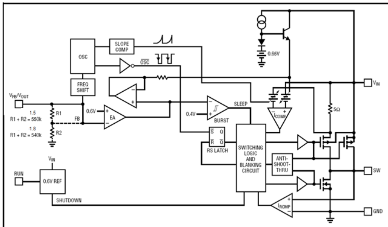
Figure2:Functional Block Diagram of TD6811B
