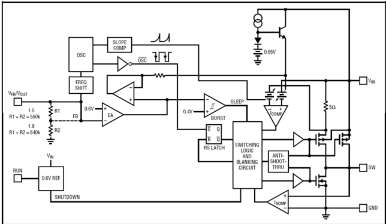
Figure2:Functional Block Diagram of TD6817
