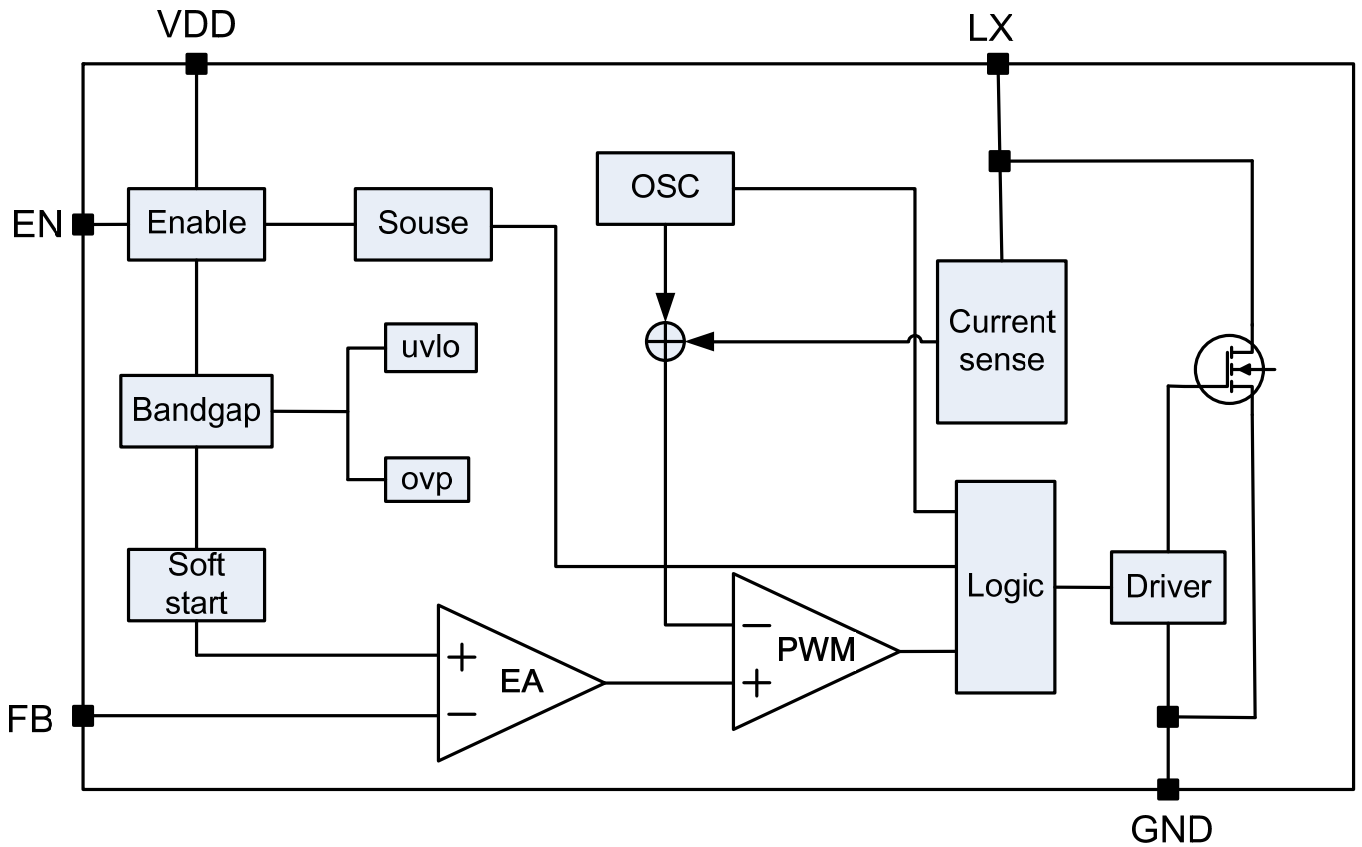
Figure 2 Function Block Diagram of TD8218
