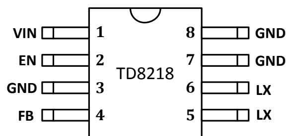
Figure1 Pin Configuration of TD8218(Top View)
