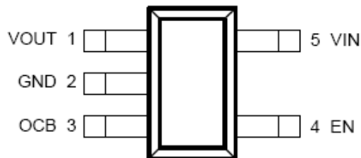
SOT-23-5(Top View) TD9516A/TD9517A
