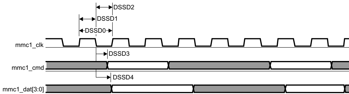
Figure 5-71. MMC/SD/SDIO in - Default Speed - Transmitter Mode
