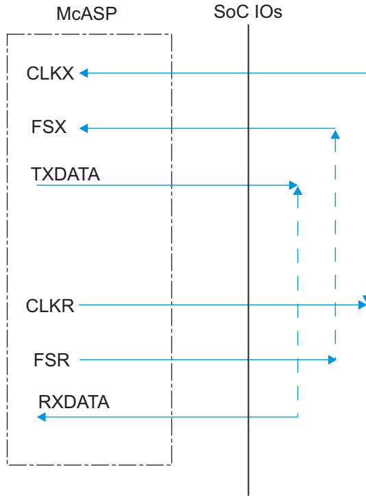
Figure 5-54. McASP1-8 CIOFIO – ASYNC Mode
