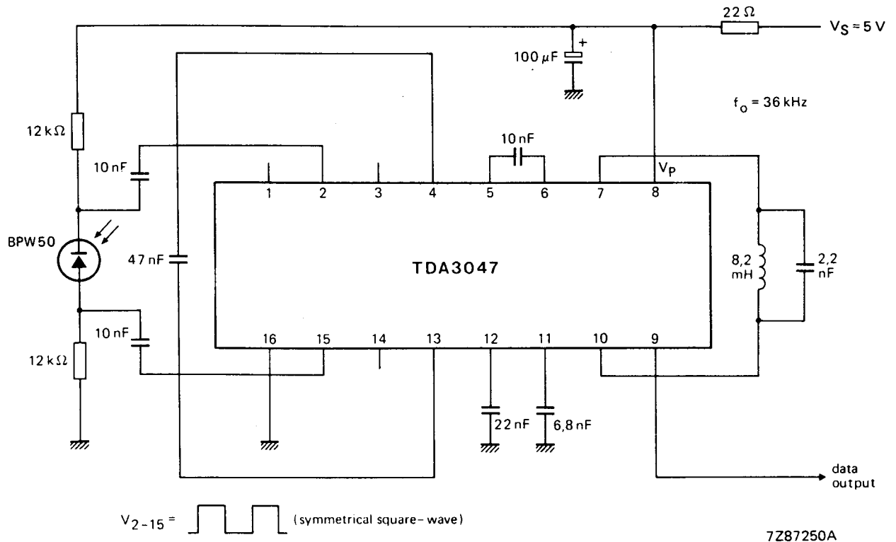
Fig. 4 Wide-band receiver with TDA3047.
