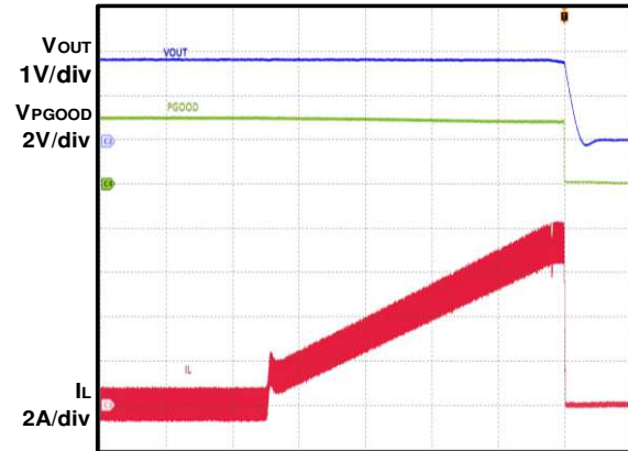
Over-Current Protection FCCM
