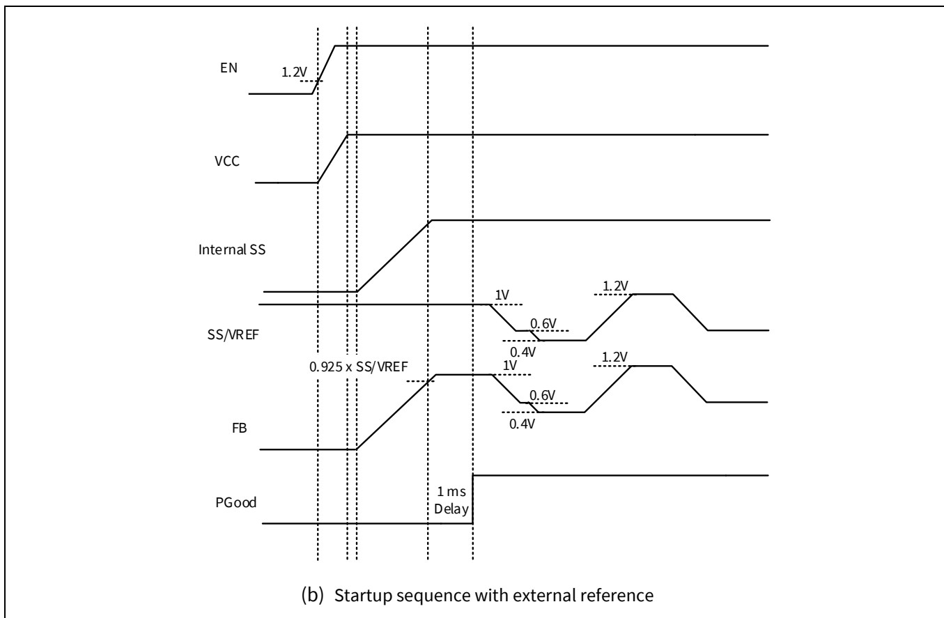
Figure 5 Startup sequence with voltage tracking and external reference
