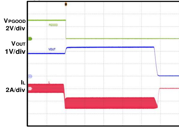
Over-Voltage Protection FCCM
