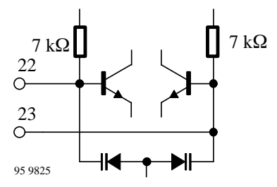
Figure 18. VCO (Pin 22-23)
