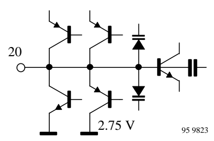
Figure 16. Loop filter (Pin 20)
