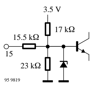
Figure 12. Standard switch (Pin 15)
