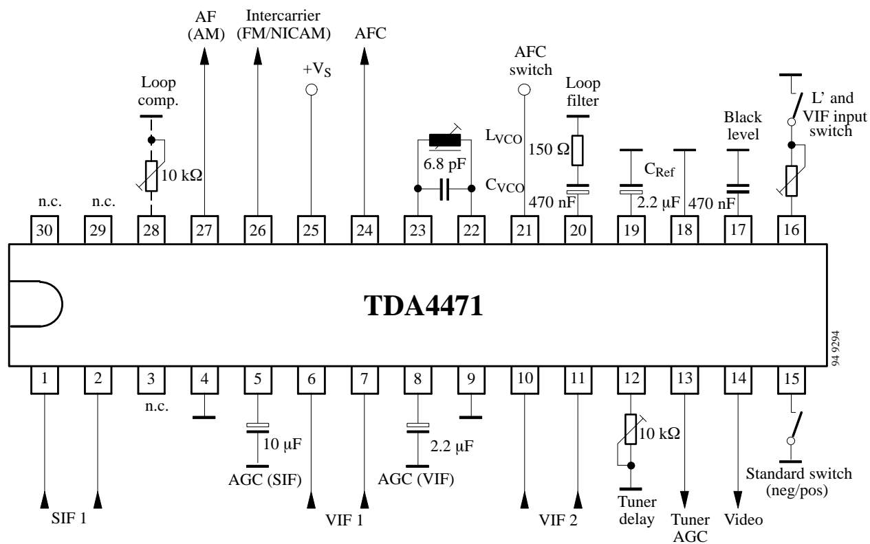
Figure 3. Test circuit
