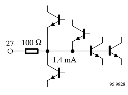
Figure 21. AF-AM output (Pin 27)
