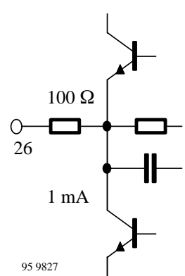
Figure 20. Intercarrier output (Pin 26)
