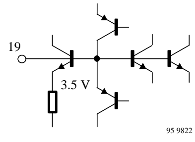
Figure 15. Internal reference voltage (Pin 19)
