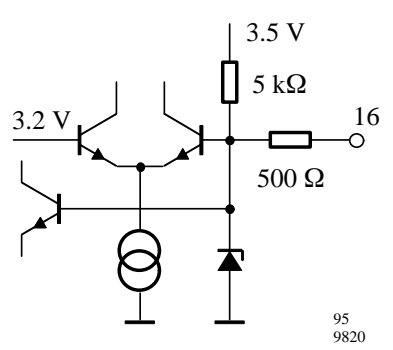
Figure 13. L'/VIF input switch (Pin 16)
