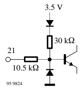
Figure 17. AFC switch (Pin 21)
