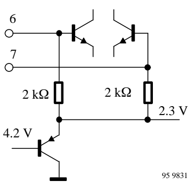
Figure 7. Video IF input (Pin 6-7)
