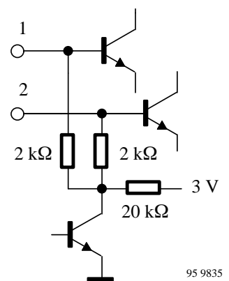
Figure 5. Sound IF inputs (Pin 1-2)
