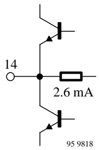
Figure 11. Video output (Pin 14)
