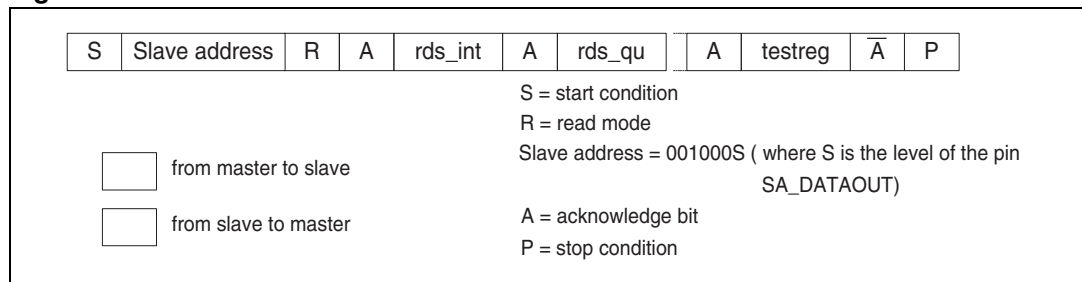
Figure 13. I 2 C read transfer
