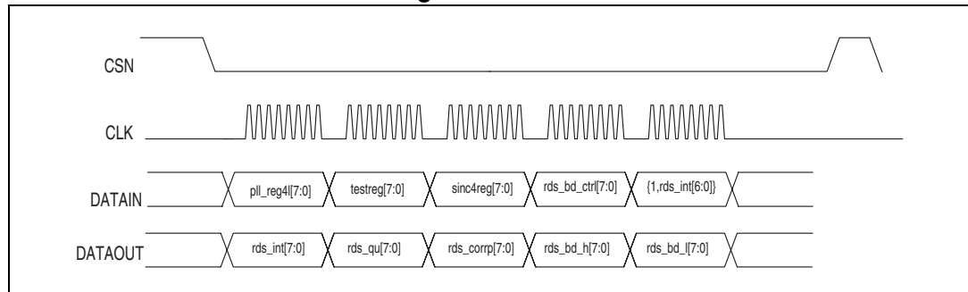
Figure 17. Write rds_int, rds_bd_ctrl and pll_reg4 registers in SPI mode, reading RDS data and related flags
