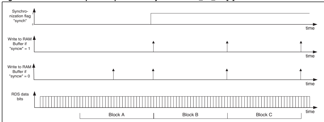
Figure 8. RAM buffer update depends on “syncw” bit rds_bd_ctrl[0]
