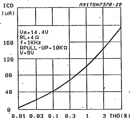
Figure 11: Clipping Detector Average Current (Pin 10) vs. Distortion
