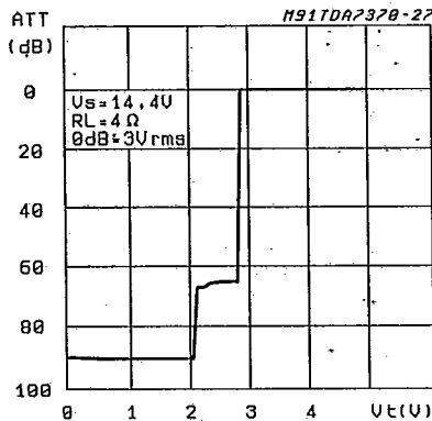
Figure 9: Stand-by Attenuation vs. Threshold Voltage
