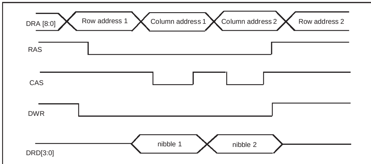
Figure 19. DRAM Write Cycle.
