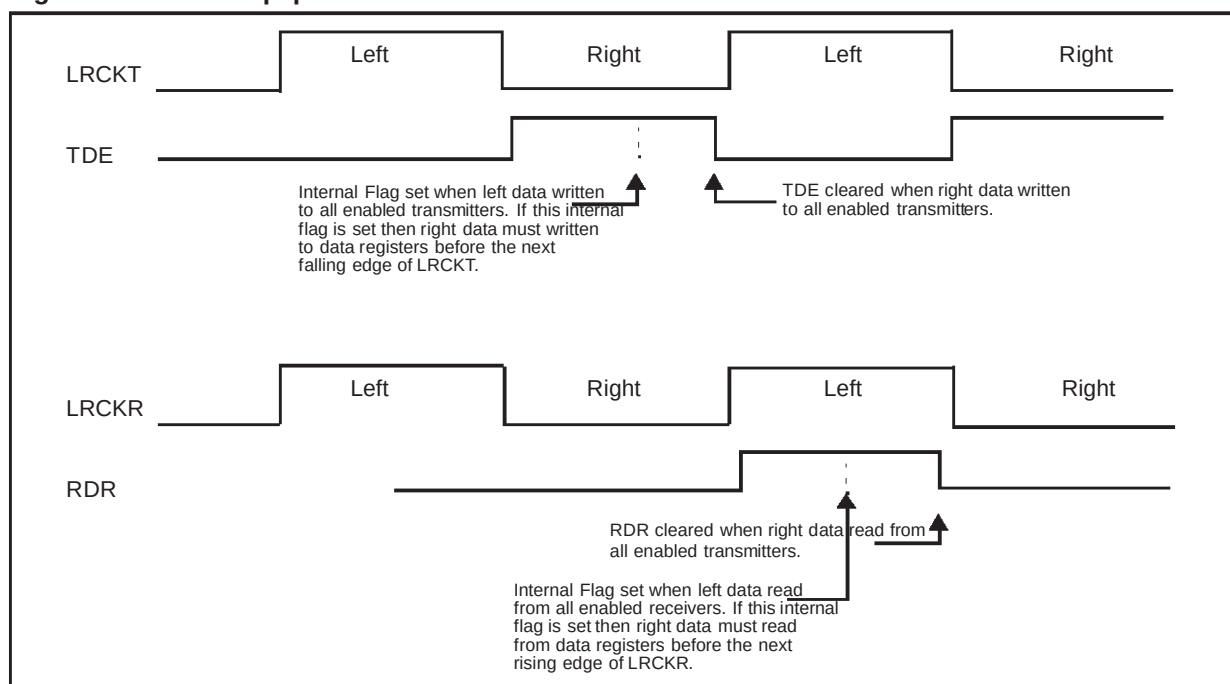
Figure 2. SAI Interrupt protocol
