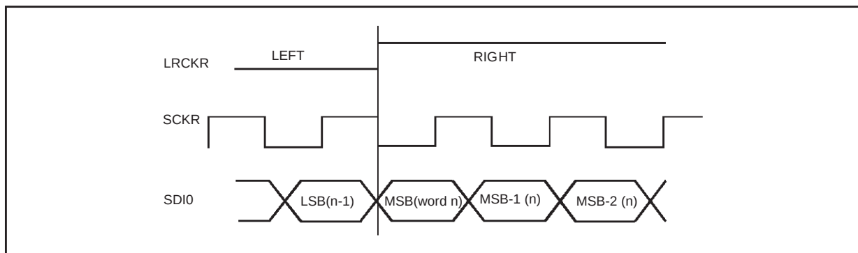
Figure 6. SAI protocol when RLRS=0; RREL=1; RCKP=1; RDIR=0.
