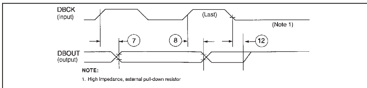
Figure 15. Debug Port DBCK Next Command After Read Register Timing.
