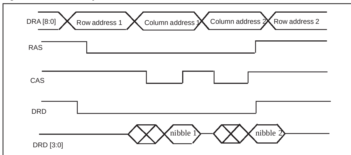
Figure 18. DRAM Read Cycle.
