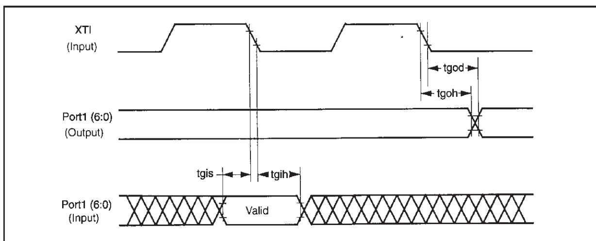
Figure 10. GPIO Timing
