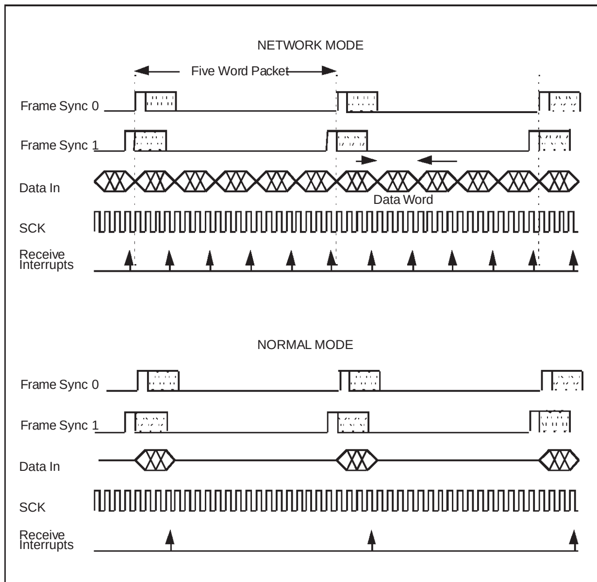
Figure 7. SSI Protocol.
