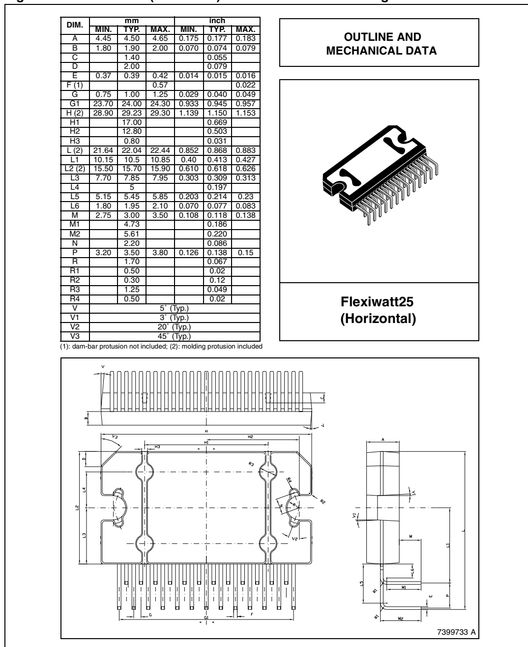
Figure 33. Flexiwatt25 (horizontal) Mechanical Data & Package Dimensions
