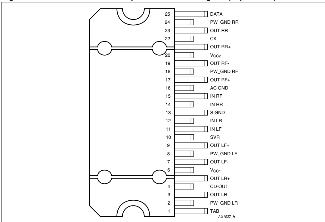
Figure 4. Flexiwatt25 horizontal pins connection diagram (Top of view)
