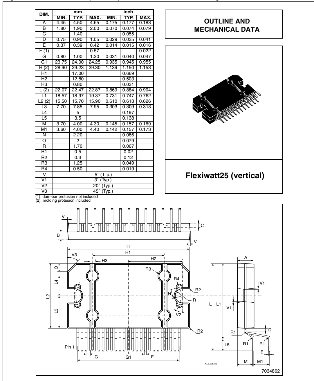
Figure 34. Flexiwatt25 (vertical) Mechanical Data &amp; Package Dimensions
