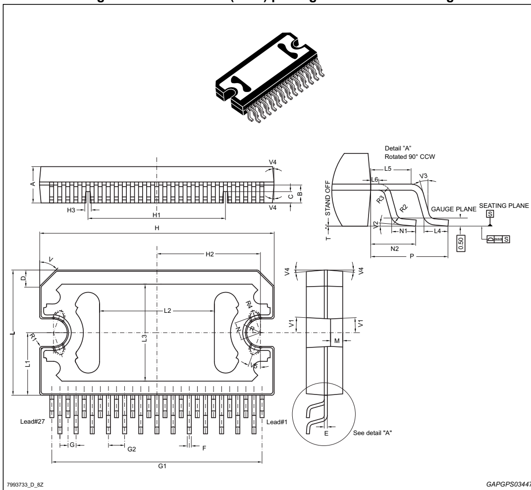
Figure 43. Flexiwatt 27 (SMD) package mechanical drawing
