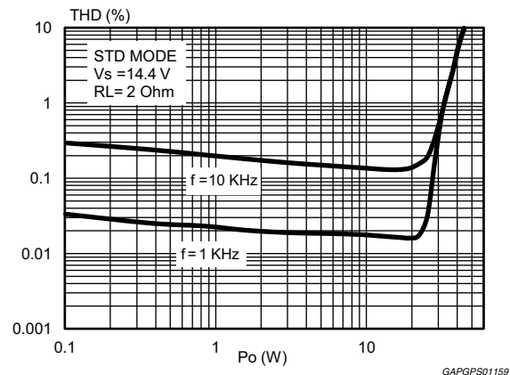
Figure 9. Distortion vs. output power (2 \Omega , STD mode)
