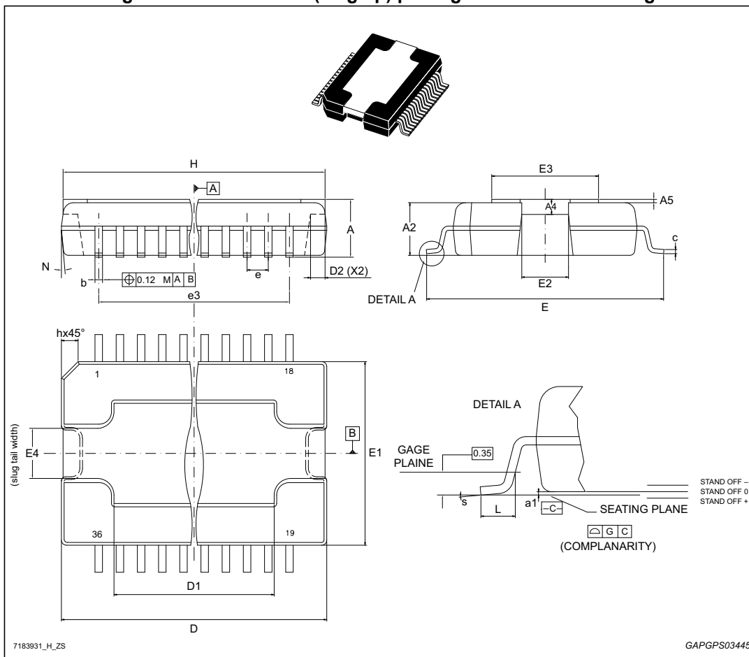
Figure 40. PowerSO-36 (slug up) package mechanical drawing
